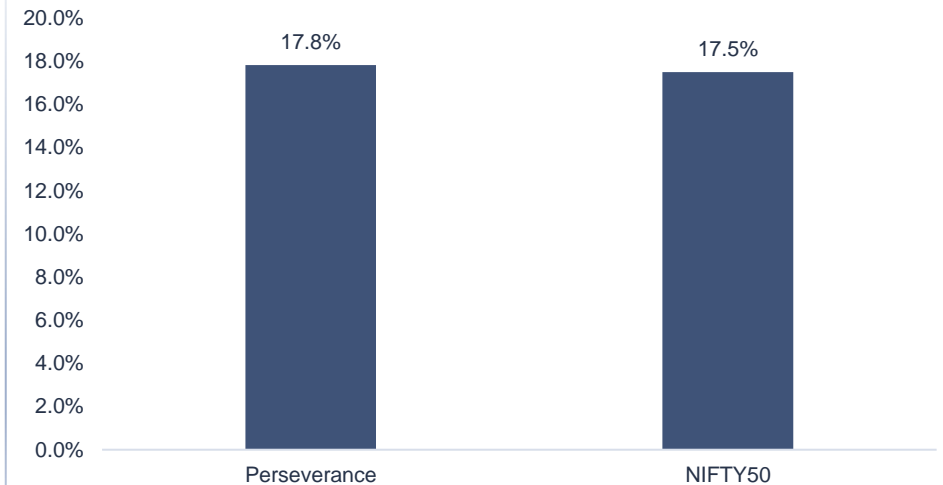
Annualized Volatility
